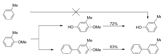
Scheme 1. Synthesis of the regioisomeric products that are unattainable from conventional toluene functionalization (for the reaction conditions, see the Supporting Information, Scheme S4).
